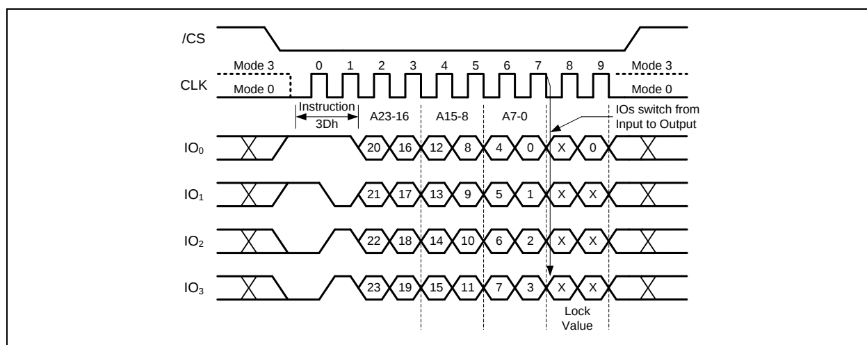
Figure 54b. Read Block Lock Instruction (QPI Mode) 32-Bit Address is required when the device is operating in 4-Byte Address Mode
